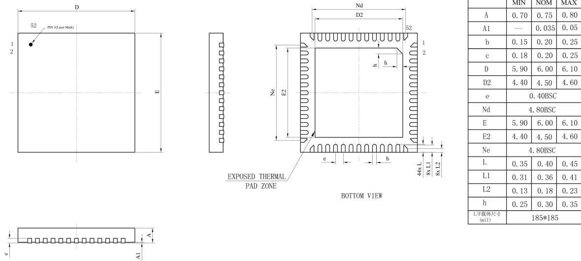
Figure 4-1 JL7012C Package
